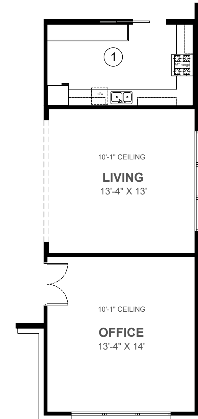
1 SECOND KITCHEN 13'-4" X 7'-8" 10' CEILING
