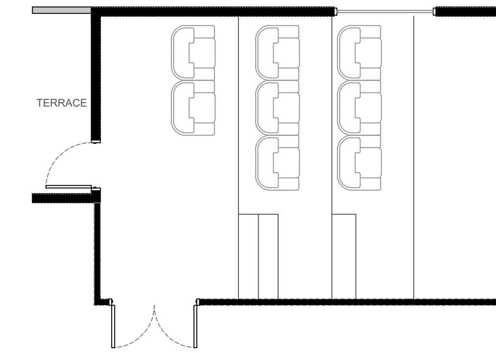
3 OPTIONAL MEDIA ROOM 20'-3" X 16'-9" 9' CEILING
