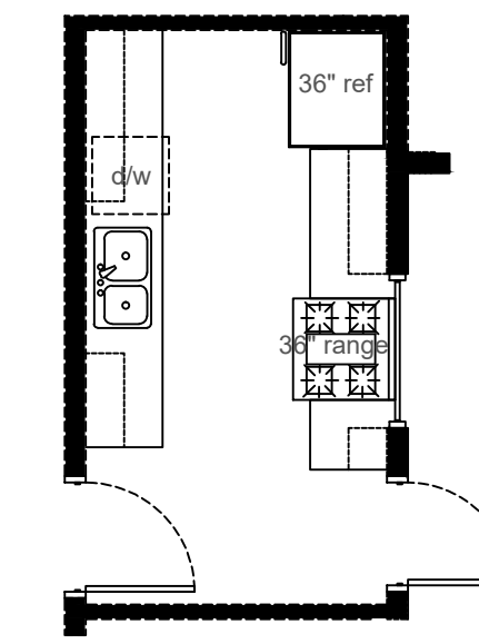
① PREP KITCHEN 7'-11" X 13'-2" 10' CEILING
