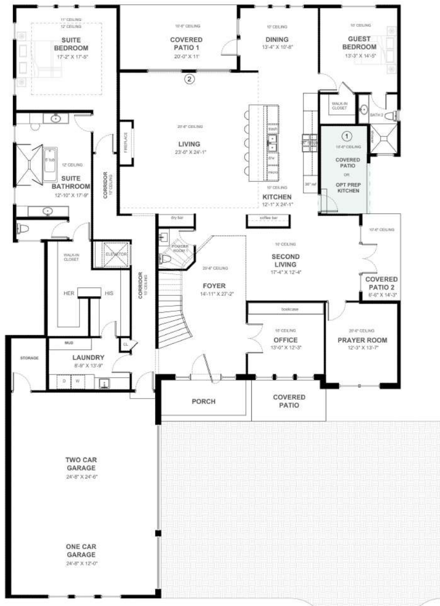
① PREP KITCHEN 7'-11" X 13'-2" 10' CEILING
