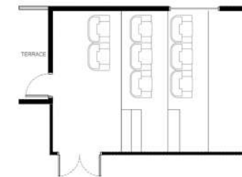
③ OPTIONAL MEDIA ROOM 20'-3" X 16'-9" 9' CEILING
